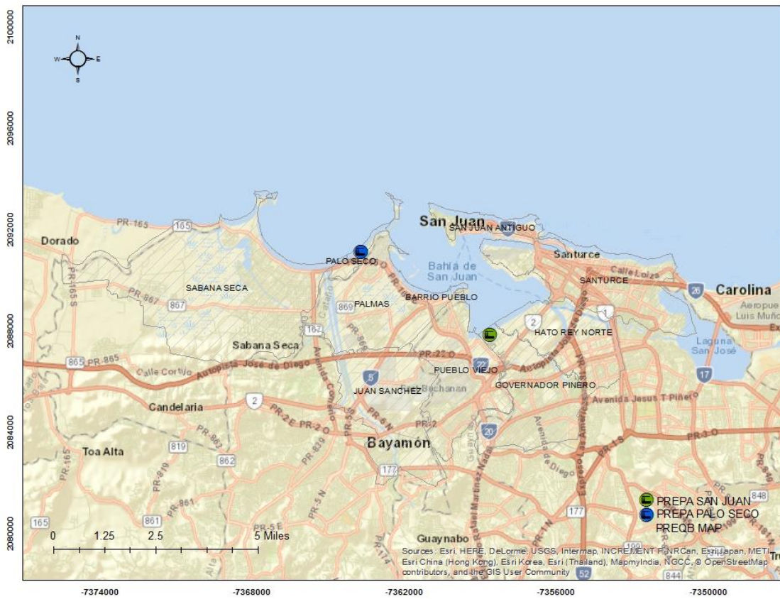
Figure 1. Includes the non-attainment area municipalities and wards. Also presents the site location for PREPA San Juan and PREPA Palo Seco.
