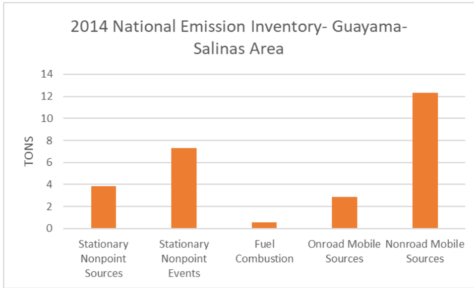
Figure 4: Shows the SO 2 emissions by sector in Guayama-Salinas Area for year 2014.
