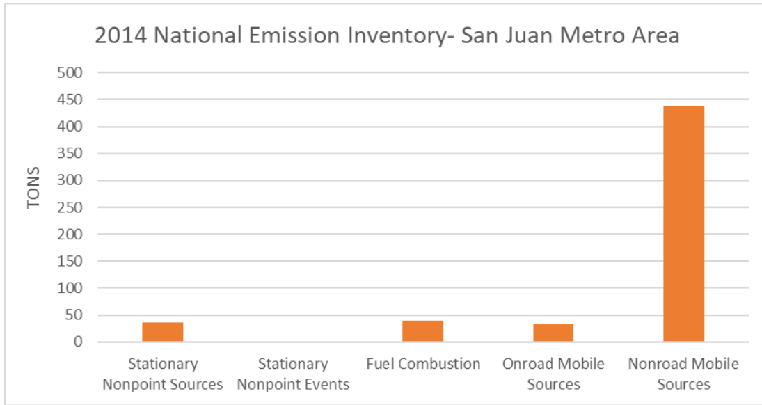
Figure 3: Shows the SO 2 emissions by sector in San Juan Metro Area for year 2014.
